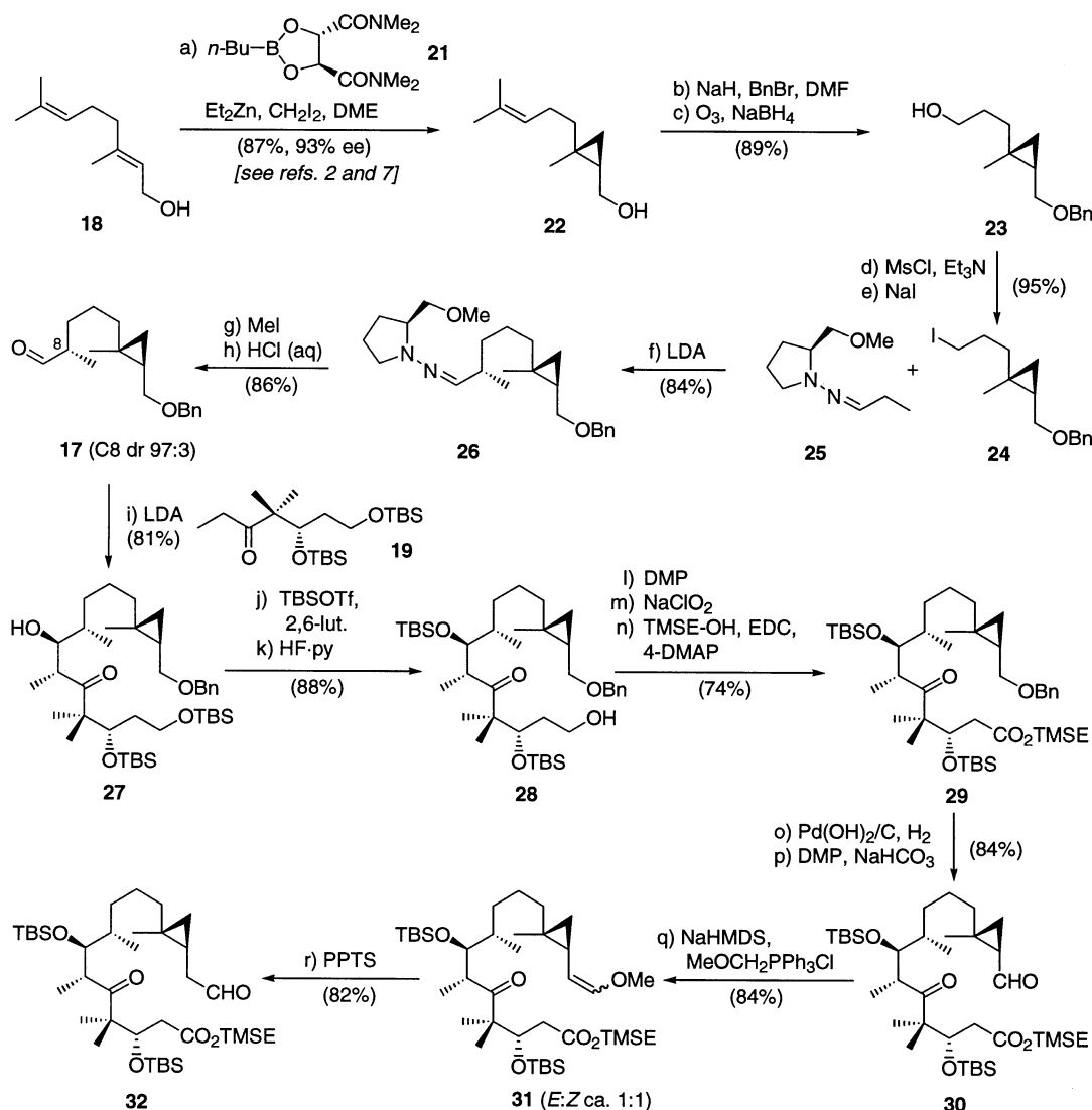
Scheme 3. Construction of aldehyde 32 . Reagents and conditions: (a) See Refs. 2 and 7; (b) \text{NaH} (1.5 equiv.), \text{BnBr} (1.5 equiv.), DMF, 0 \rightarrow 25^\circ\text{C} , 12 h; (c) \text{O}_3 , \text{CH}_2\text{Cl}_2/\text{MeOH} 4:1, -78^\circ\text{C} , 21 min; then \text{NaBH}_4 (3.0 equiv.), -78 \rightarrow 25^\circ\text{C} , 1 h, 89% for two steps; (d) \text{MsCl} (1.3 equiv.), \text{Et}_3\text{N} (1.5 equiv.), \text{CH}_2\text{Cl}_2 , 25^\circ\text{C} , 1 h; (e) \text{NaI} (3.0 equiv.), acetone, reflux, 40 min, 95% for two steps; (f) \text{LDA} (1.4 equiv.), 25 (1.3 equiv.), THF, 0^\circ\text{C} , 6 h; then 24 , -98 \rightarrow -10^\circ\text{C} , 14 h, 84%; (g) \text{MeI} , 60^\circ\text{C} , 3 h; (h) 3\text{N HCl} :pentane 1:1, 25^\circ\text{C} , 3 h, 88% for two steps; (i) \text{LDA} (2.4 equiv.), 19 (2.3 equiv.), THF, -78^\circ\text{C} , 1 h; then -40^\circ\text{C} , 0.5 h; then 17 at -78^\circ\text{C} , 5 min, 81%; (j) \text{TBSOTf} (2.0 equiv.), 2,6-lutidine (3.0 equiv.), \text{CH}_2\text{Cl}_2 , -20^\circ\text{C} , 1 h; (k) \text{HF}\cdot\text{py} , pyridine, THF, 25^\circ\text{C} , 4 h, 88% for two steps; (l) \text{DMP} (2.5 equiv.), \text{NaHCO}_3 (2.5 equiv.), \text{H}_2\text{O} , \text{CH}_2\text{Cl}_2 , 25^\circ\text{C} , 1 h; (m) \text{NaClO}_2 (3.1 equiv.), \text{NaH}_2\text{PO}_4 (2.1 equiv.), 2-methyl-2-butene (74 equiv.), t\text{-BuOH} , THF, \text{H}_2\text{O} , 25^\circ\text{C} , 1 h; (n) 2-(trimethylsilyl)ethanol (4.0 equiv.), \text{EDC} (1.5 equiv.), 4-DMAP (0.1 equiv.), DMF, 25^\circ\text{C} , 14 h, 74% for three steps; (o) 20% \text{Pd}(\text{OH})_2/\text{C} , \text{H}_2 (1 atm), \text{EtOH}/\text{EtOAc} 1:1, 25^\circ\text{C} , 1 h; (p) \text{DMP} (2.5 equiv.), \text{NaHCO}_3 (2.5 equiv.), \text{H}_2\text{O} , \text{CH}_2\text{Cl}_2 , 25^\circ\text{C} , 1 h, 84% for two steps; (q) \text{MeOCH}_2\text{PPh}_3\text{Cl} (3.0 equiv.), \text{NaHMDS} (2.8 equiv.), THF, -40 \rightarrow -10^\circ\text{C} , 2 h, 84%; (r) \text{PPTS} (8.0 equiv.), dioxane: \text{H}_2\text{O} 9:1, 70^\circ\text{C} , 6 h, 82%. 4-DMAP, 4-(dimethylamino)pyridine; DME, 1,2-dimethoxyethane; DMP, Dess–Martin periodinane; EDC, 1-(3-dimethylaminopropyl)-3-ethylcarbodiimide hydrochloride; \text{HF}\cdot\text{py} , hydrogen fluoride–pyridine complex; \text{NaHMDS} , sodium hexamethyldisilazide; PPTS, pyridinium para-toluenesulfonate; TMSE, 2-trimethylsilyl ethyl.
