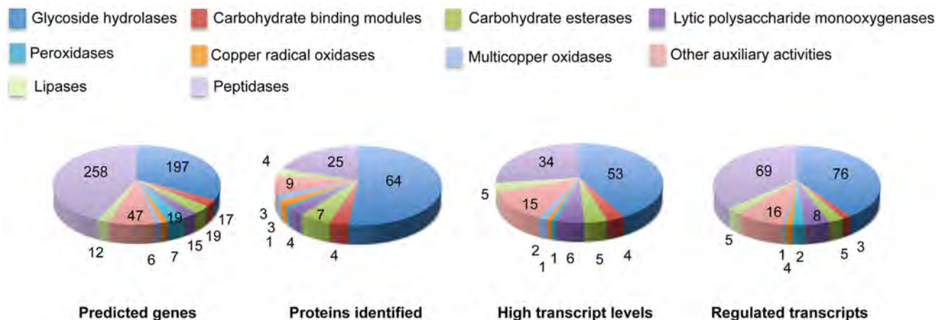
Figure 6. Number and expression of genes likely involved in lignocellulose degradation. The number of genes encoding mass spectrometry-identified proteins was limited to those matching \geq 2 unique peptides after 5–9 days growth in media containing NELP or ELP. RPKM values >100 for RNA derived from these cultures were arbitrarily selected as the threshold for high transcript levels. Genes designated as 'regulated' showed significant accumulation ( p < 0.05 ; >2-fold) in NELP or ELP relative to glucose containing media. Methods and complete data are presented in Text S1 and Dataset S2. doi:10.1371/journal.pgen.1004759.g006
