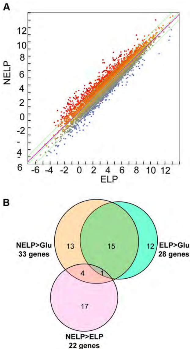
Figure 7. P. gigantea transcriptome. Scatterplot (A) shows the distribution of RNA-seq RPKM values (log 2 ) for 11,376 P. gigantea genes when grown on basal salts containing acetone-extracted loblolly pine wood (ELP) or non-extracted loblolly pine wood (NELP). Lines define 2-fold borders and best fit regression. Darkened points represent 44 transcripts accumulating >4-fold at p<0.01. Venn diagram (B) illustrates genes with RPKM signals >10 and upregulated >4-fold in NELP relative to ELP. Twenty-two genes showed significant transcript accumulation in NELP relative to ELP suggesting potential response to resin and pitch content. Under these stringent thresholds (p<0.01; >4-fold), only one gene, a MCO model Phlgi1_129839, showed significant transcript accumulation in ELP relative to NELP. Additional detail appears in Tables 1–3. Detailed methods and complete data are presented in Text S1 and Dataset S2.
