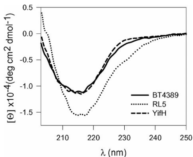
FIGURE 7. CD spectra of the RL5 (rumen metagenome), YifH ( E. coli ), and BT4389 ( B. thetaiomicon ) proteins.
